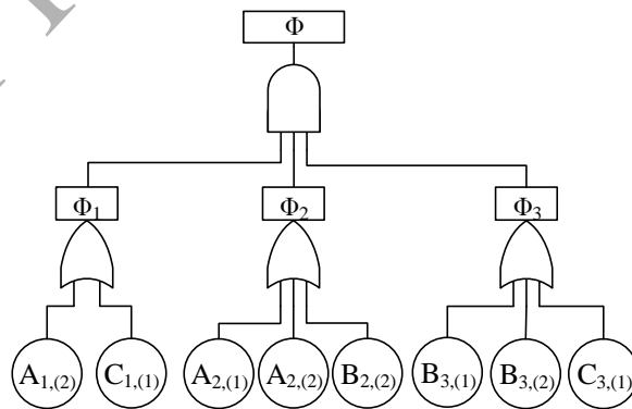
Fig. 2. The MFT model for the example system.
