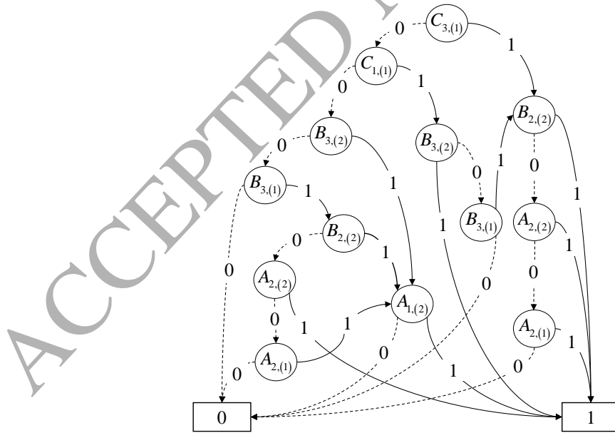
Fig. 8. The system BDD model for the example PMS.
