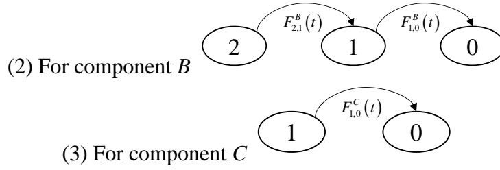
Fig. 1. The state transition graphs for components in the example system.
