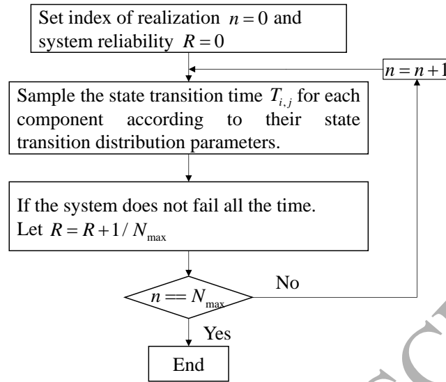
Fig. 19. Monte Carlo simulation procedure
