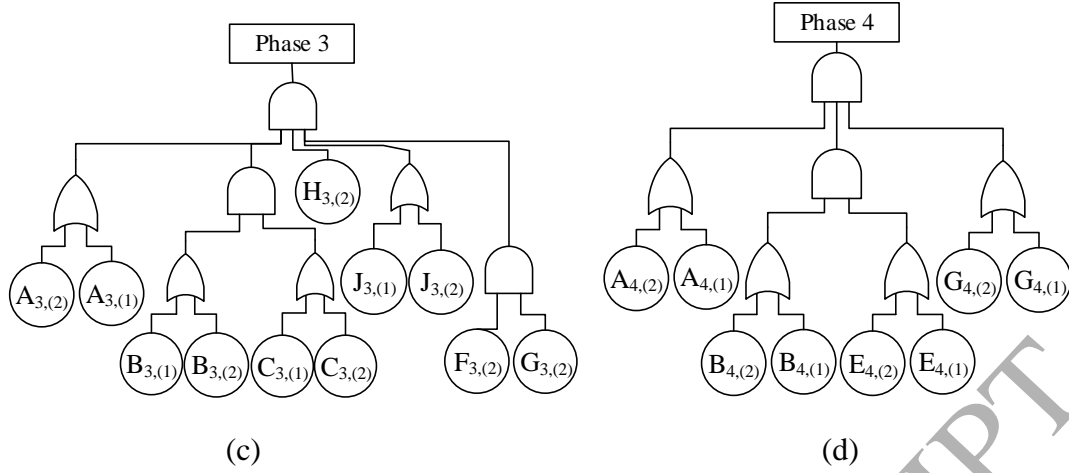
Fig. 17. The fault tree model for each phase of the AOCS.
