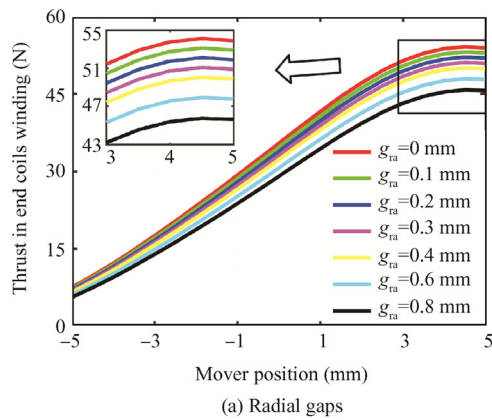
(a) Radial gaps
