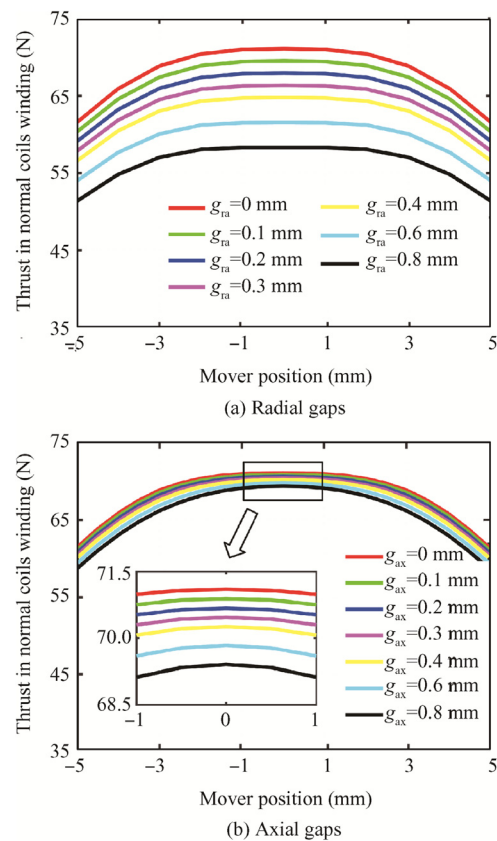
Fig. 11 Effect of gaps on thrust in normal coils winding.
