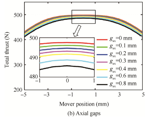
Fig. 13 Effect of gaps on total thrust.
