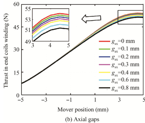
Fig. 12 Effect of gaps on thrust in end coils winding.
