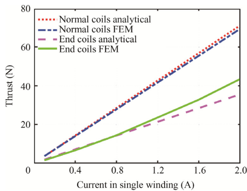
Fig. 8 Validation of thrust.
