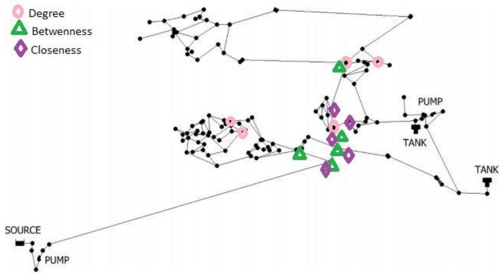
Figure 6. Distribution of sensor node locations in a WDN network(BWSN) based on the maximization of degree, betweenness and closeness centrality metrics which are mostly located in the inner side of the network
